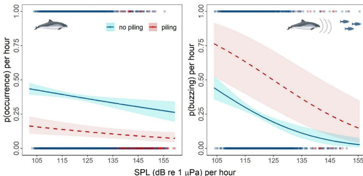
Plate 6.2 [Left] The probability of harbour porpoise presence in relation to the SPL (Red = during piling, Blue = outside of piling time, and [Right] the probability of buzzing activity per hour in relation to the SPL (Red = during piling, Blue = outside of piling)
