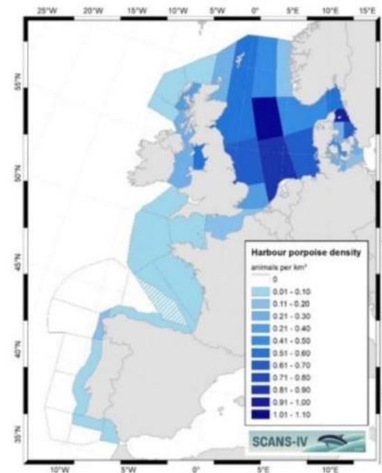
Plate 5.5 Estimated density in each survey block for harbour porpoise from SCANS-IV (Gilles et al., 2023)
